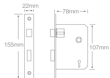
QS5757/4L Stainless steel forend – four lever 57mm backset 57mm centre
