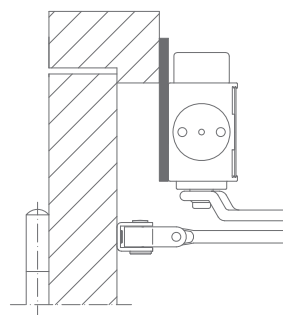
QS7704 | Drop plate For fixing when the door closer cannot be installed directly onto the door frame
