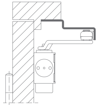
QS7708/B | Parallel arm bracket For the installation of the arm assembly parallel to the door frame
