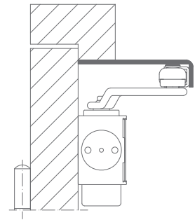
QS7708/A | Parallel arm bracket For the installation of the arm assembly parallel to the door frame
