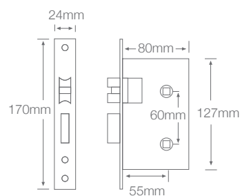
QS6055/5 Bathroom lock 55mm backset 60mm centre
