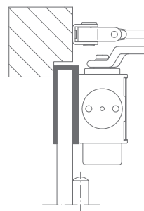
QS7702 | Glass door shoe For the installation of the door closer to all-glass doors (maximum 10mm glass thickness)
