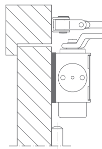
QS7710 | Mounting backplate For the installation of the door closer on fireproof and smoke control doors
