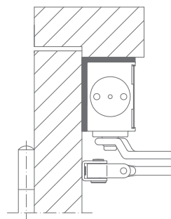
QS7705 | Angle bracket For transom fixing of the door closer on the push side in case of a deep lintel of the door
