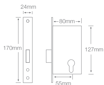
QS6055/4 Deadbolt 55mm backset
