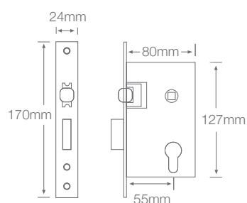
QS6055/3 Cylinder adjustable rollerbolt and deadbolt 55mm backset 60mm centre
