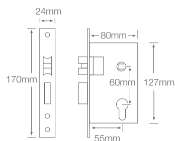
QS6055/1 Latch and deadbolt 55mm backset 60mm centre
